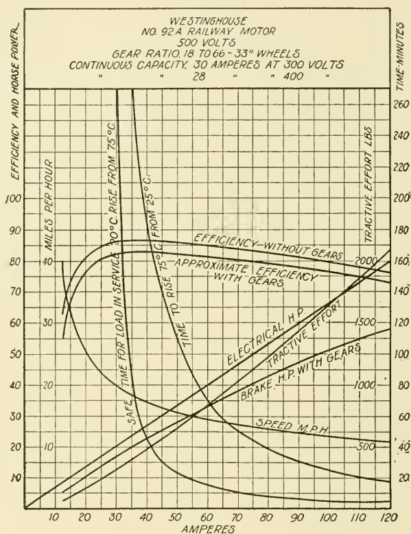
Fig. 47. Characteristic Curves—Westinghouse Railway Motor
